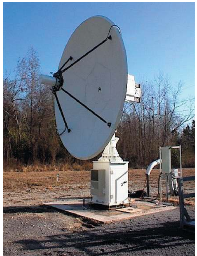
DASS Proof-of-Concept Local User Terminal at NASA's SARLAB
